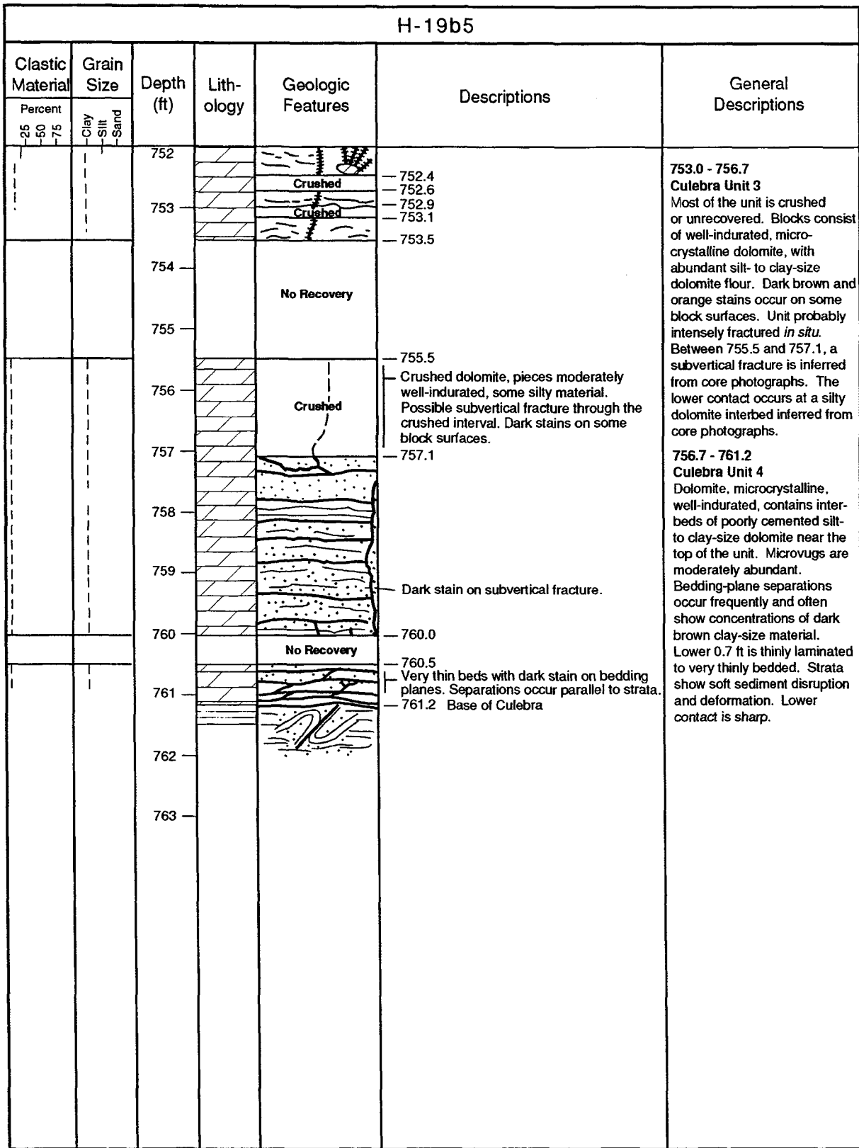
Figure 3-6b. Detailed geologic description of the Culebra interval from H-19b5.
