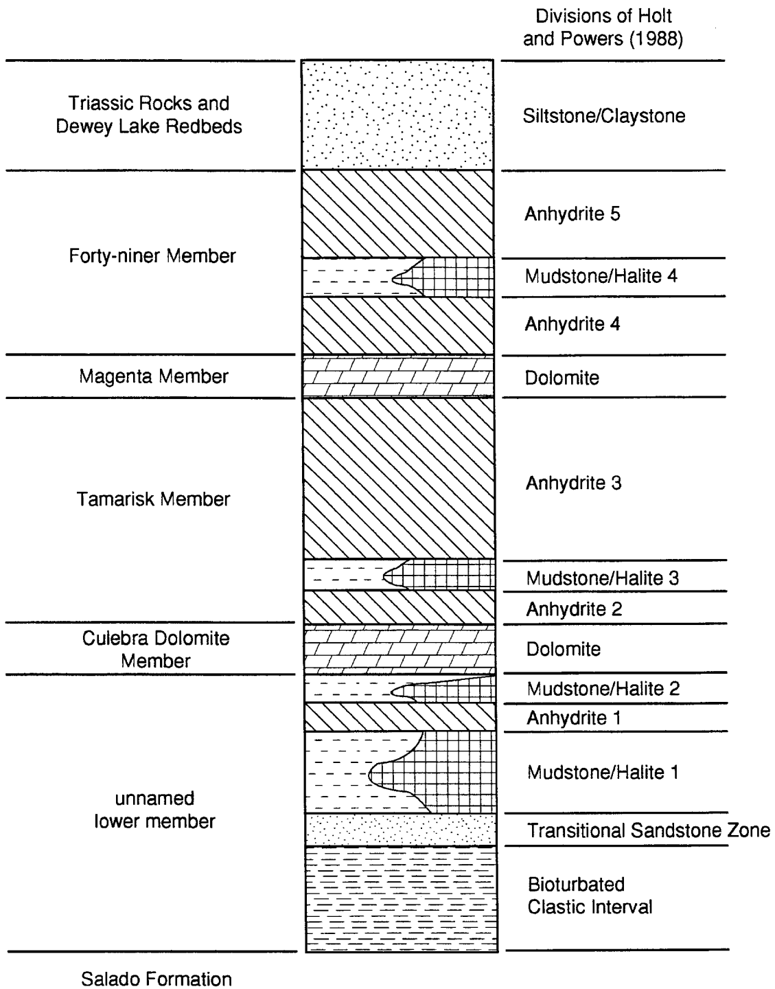
Figure 3-9. Rustler stratigraphy.
